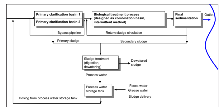
Fig 2. The wastewater treatment plant with new operation procedures for 40,000 inhabitants
