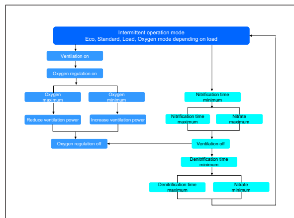
Fig 6. Nitrate controlled regulation
