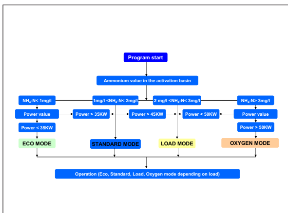
Fig 5. Operating mode of the module, Load classification.
