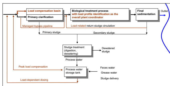
Fig 1. Original situation at the wastewater treatment plant Felsalbe
