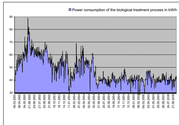
Fig 9. Power consumption of the biological treatment process (Feb 2003 to Sept 2005)
