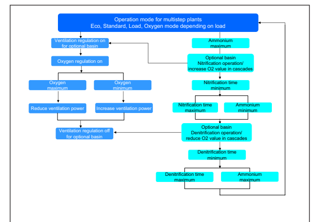
Fig 7. Ammonium controlled regulation
