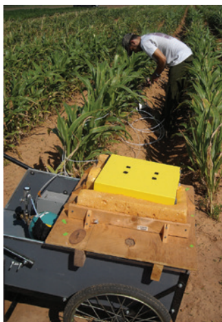
Student technician Tony Guajardo places the soil flux chamber on a soil collar to begin measurement of GHGs from the soil.
