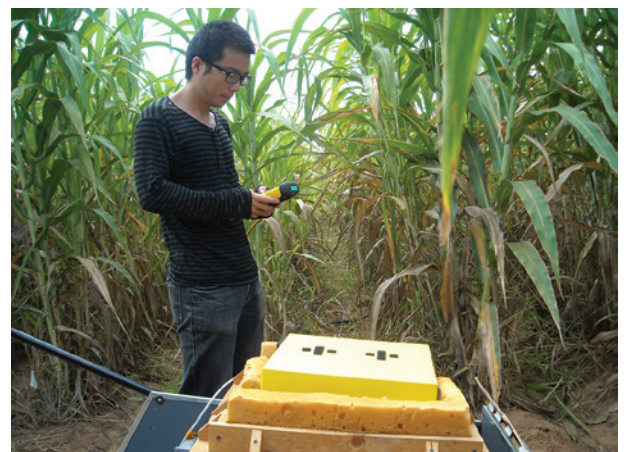
Graduate researcher Yong Wang uses a wireless PDA to control operations and monitor results from the mobile-FTIR in a sorghum field.
