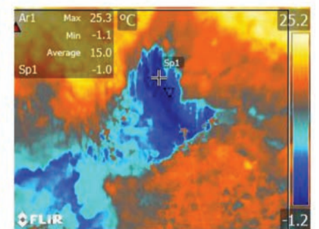
Natural thaw subsidence along ice wedges on the terraces of Chara river (August 2013)
