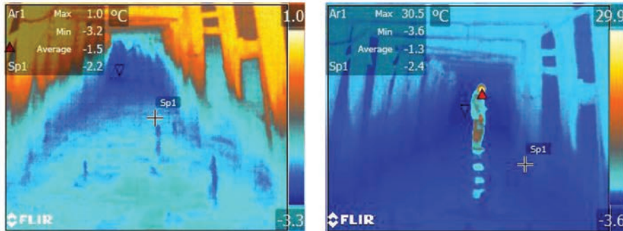
Thermal imaging can also be used in support of mining and tunnel construction works in permafrost areas. (Udokan Ridge tunnel works, similar to the Kodar tunnel works)
