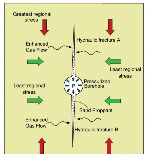
Figure 2: Schematic illustration of hydraulic fracture produced by pressurizing a borehole with water. When fluid pressure P is made to exceed the least regional stress, a pair of hydraulic fractures propagate some metres away from the borehole wall, parallel to the greatest regional stress, increasing the effective cross-sectional area over which gas can flow into the hole from the low permeability shale. A sandy proppant is carried by the fracturing fluid to prevent the crack from closing when the water pressure is reduced to allow the gas to flow out of the pores of the rock.
