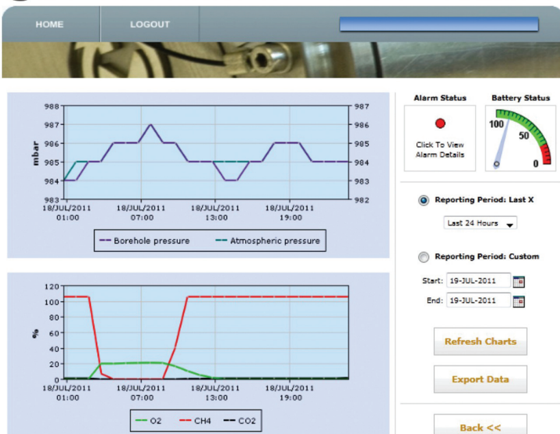
Figure 7: Website interface to Gasclam M2M telemetry showing test data from prior 24 hours and indicating whether an alarm condition has been breached ( http://www.salamander-group.co.uk/ ).
