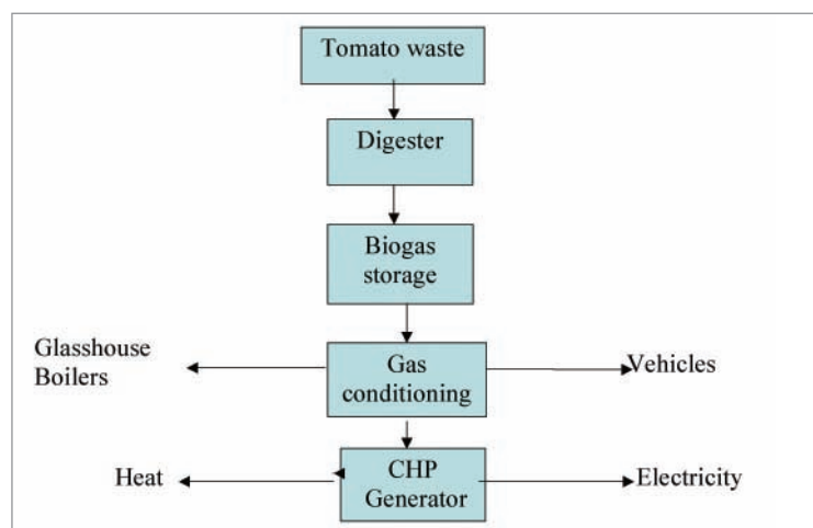
Figure 4: AD/CHP System
