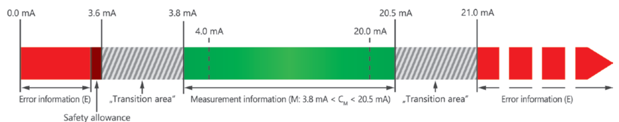
Illustration of limit ranges 4-20mA EN
