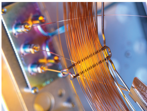
GC column for Siloxane gas mixtures analysis - NPL
