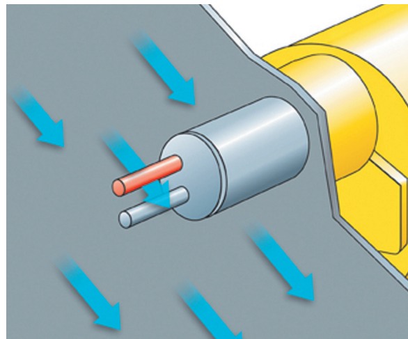
Figure 4: Thermal Dispersion Sensing Cut-Away
